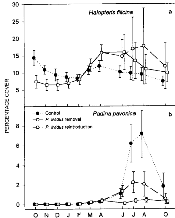
Fig. 3. Time course of the percentage cover of (a) Halopteris filicina and (b) Padina pavonica during the experiment. Bars are standard errors ( n = 10 for control plots and for removal plots until April; n = 5 for removal and reintroduction plots thereafter).
